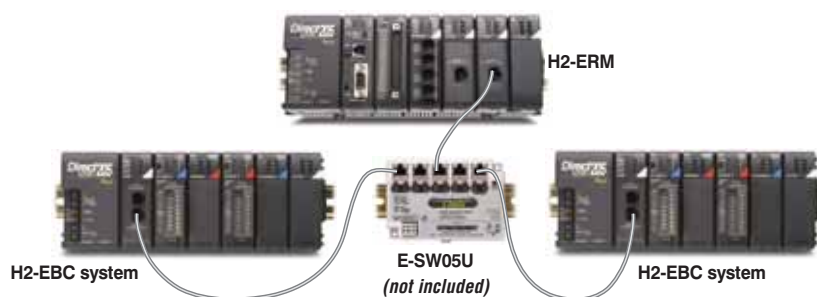
Example of an Ethernet remote I/O system using an H2-ERKIT-2. CPU, bases, I/O modules, Ethernet hub, etc. are sold separately.
